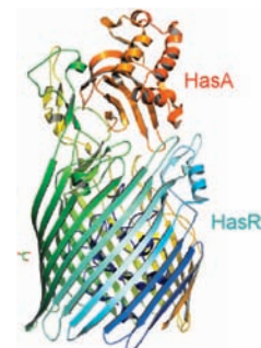
Figure 4. Ribbon representation of the S. marcescens hemophore, HasA (red), bound to its outer membrane receptor protein HasR (blue) (PDB code 3CSN). 33
