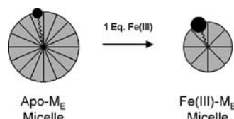
Figure 11. Coordination of Fe(III) could give M_E a larger headgroup area:tail volume ratio such that a smaller micelle is formed. 107 Reproduced from ref 107.
